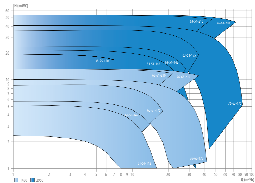
Performance Curves - Complete DanPumps S-FP Range - 50 Hz with max. and min. impeller diameter
